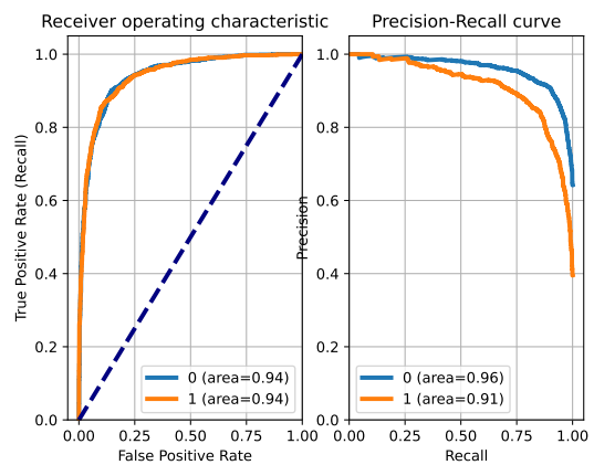
(b) ROC Curve and PR Curve
